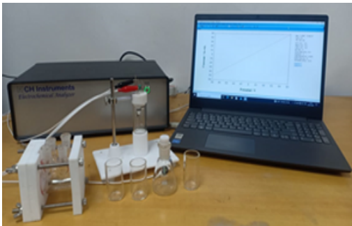
Electrochemical Workstation
