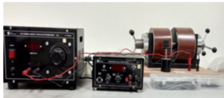
Four Probe Hall Measurement
