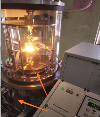
Sputtering/Evaporation
